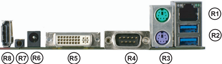
Standard LI91EHG3 Rear IO Ports
