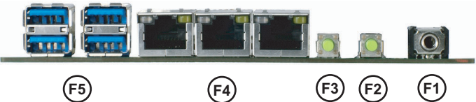
Standard LI91EHG3 Front IO Ports
